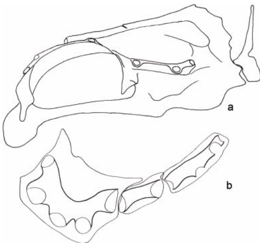
Fig. 26. Lamprologus teugelsi , n.sp., AMNH 233612: (a) neurocranium and first vertebra; (b) lachrymal and adjacent infraorbitals.
