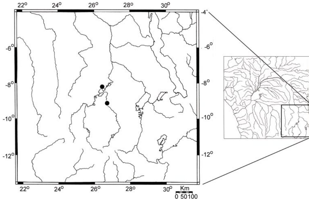
Fig. 20. Collection localities of Lamprologus symoensi .
