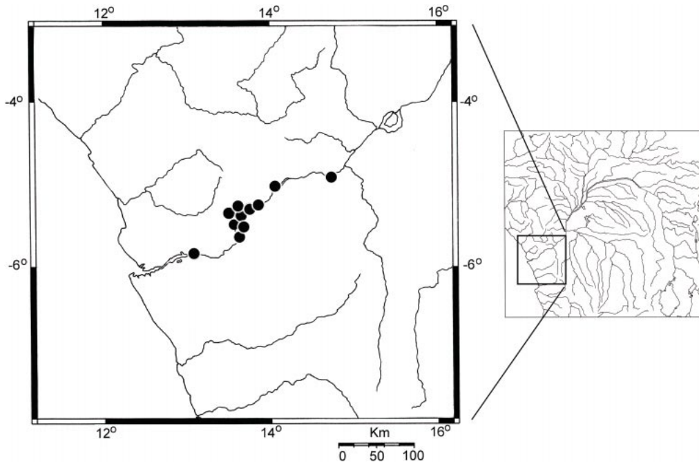
Fig. 31. Collection localities of Lamprologus tigripictilis , n.sp.
