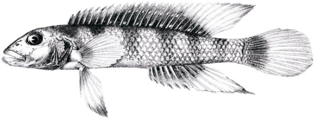
Fig. 15. Lamprologus weneri , male, 123 mm TL, modified from Poll (1959).
