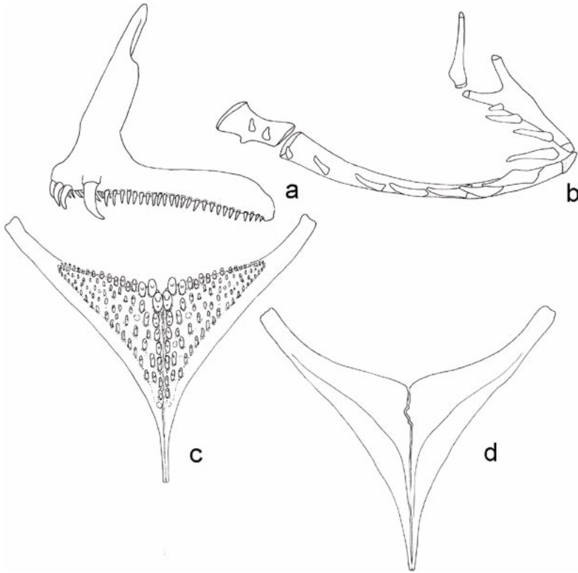
Fig. 29. Lamprologus tigripictilis , n.sp., USNM 216359: (a) premaxilla; (b) first gill arch; (c) lower pharyngeal jaw dorsal view; (d) lower pharyngeal jaw ventral view.
