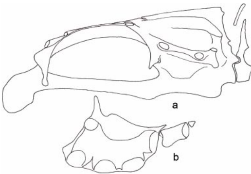
Fig. 30. Lamprologus tigripictilis , n.sp., USNM 216359: (a) neurocranium, first vertebra, and supraneural; (b) lachrymal and adjacent infraorbitals.
