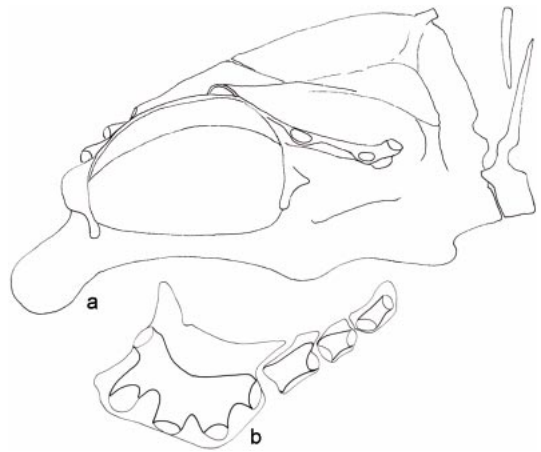
Fig. 7. Lamprologus congoensis , MRAC 118154: (a) neurocranium, first vertebra, and supraneural; (b) lachrymal and adjacent infraorbitals.
