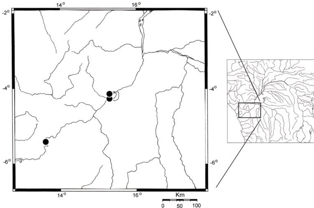
Fig. 27. Collection localities of Lamprologus teugelsi , n.sp.
