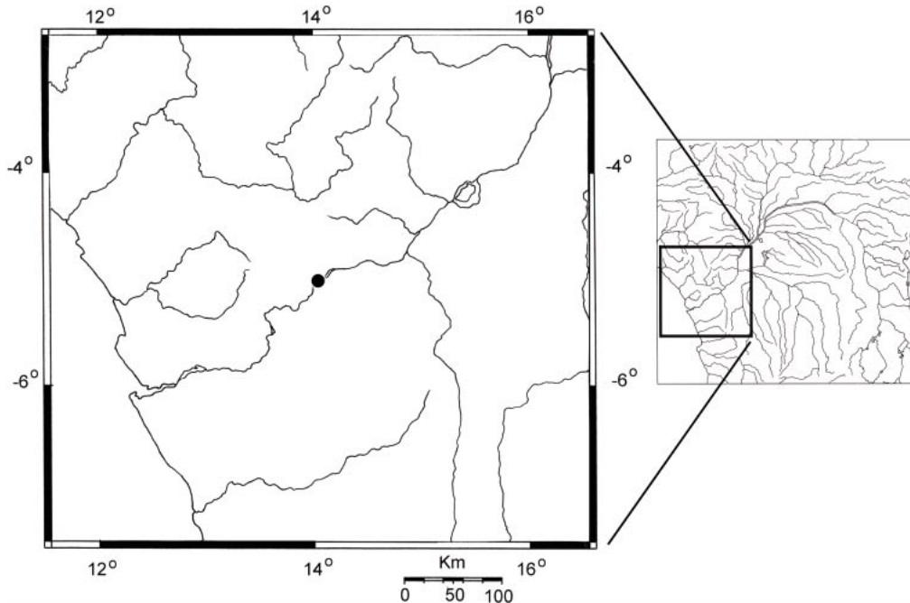
Fig. 23. Collection localities of Lamprologus lethops .
