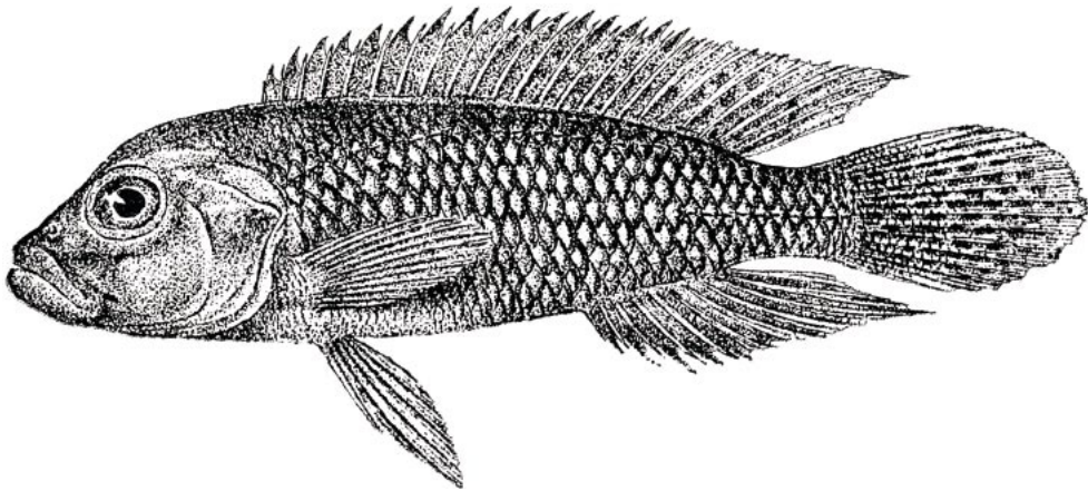
Fig. 9. Lamprologus tumbanus , male, 72 mm TL, modified from Boulenger (1899a).
