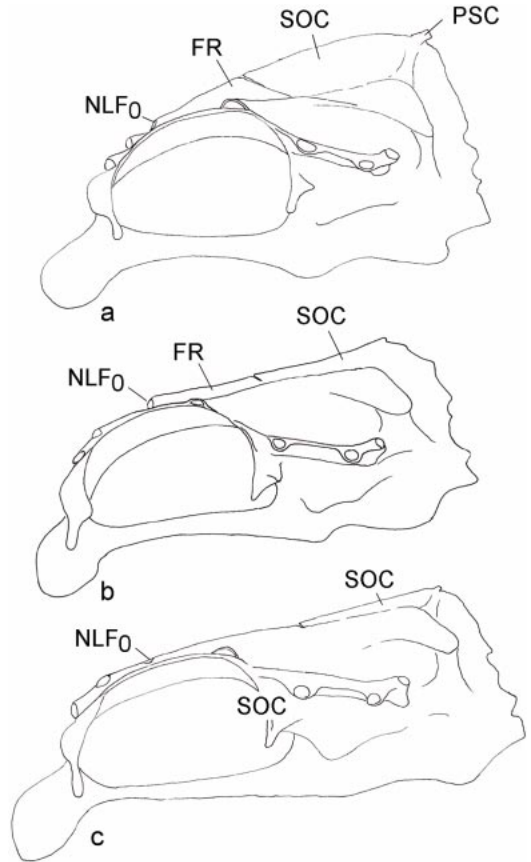
Fig. 2. Schematic of various manifestations of supraoccipital crest and frontal ridge: (a) Elevated supraoccipital crest continuous with frontal ridge to neurocranial lateral line foramen 0; (b) low supraoccipital crest continuous with frontal ridge to neurocranial lateral line foramen 0; (c) low supraoccipital crest, no frontal ridge extending to neurocranial lateral line foramen 0.
