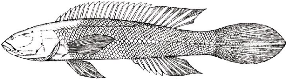
Fig. 21. Lamprologus lethops holotype, MCZ 50248, male, 26 mm SL, drawn by Patricia Wynne.
