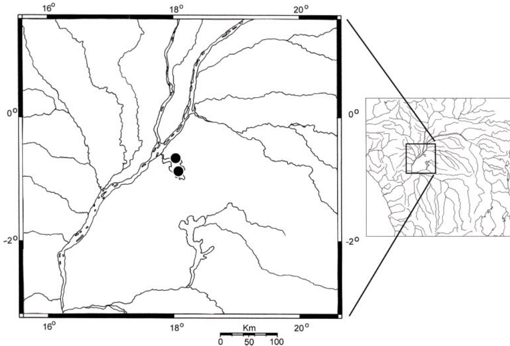
Fig. 11. Collection localities of Lamprologus tumbanus .
