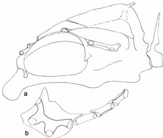
Fig. 10. Lamprologus tumbanus , MRAC 100851–53: (a) neurocranium and first vertebra; (b) lachrymal and adjacent infraorbitals.
