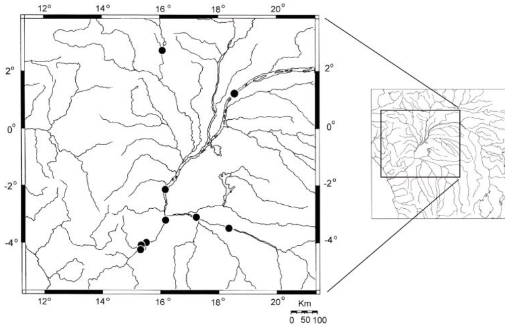
Fig. 8. Collection localities of Lamprologus congoensis .
