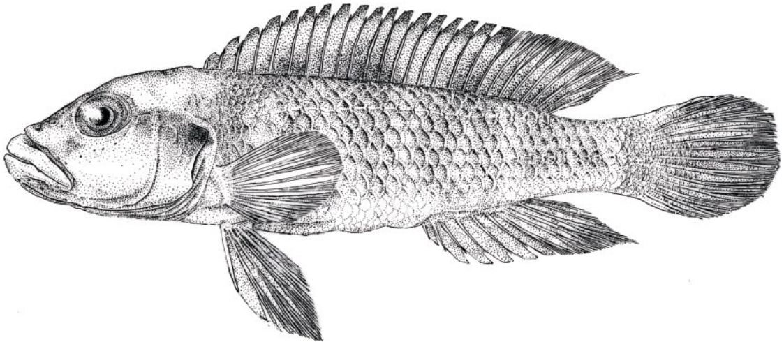
Fig. 24. Lamprologus teugelsi , n.sp., holotype, AMNH 233611, female, 60 mm SL, drawn by Ian Hart.
