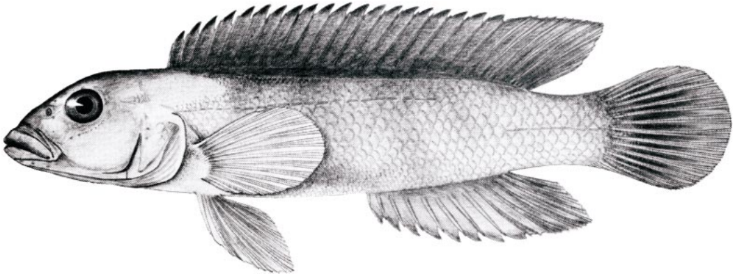
Fig. 18. Lamprologus symoensi holotype, MRAC 79001.6283, male, 53.5 mm SL, modified from Poll (1976).
