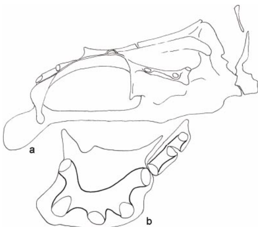
Fig. 16. Lamprologus weneri , MRAC 104004–27: (a) neurocranium and first vertebra; (b) lachrymal and adjacent infraorbitals.
