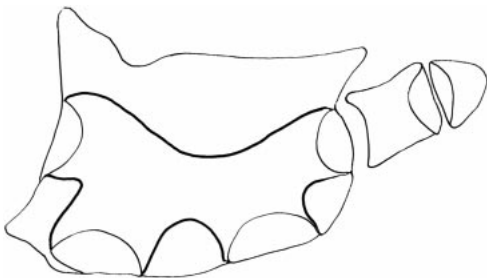
Fig. 22. Lamprologus lethops paratype, MCZ 50249: lachrymal and adjacent infraorbitals.
