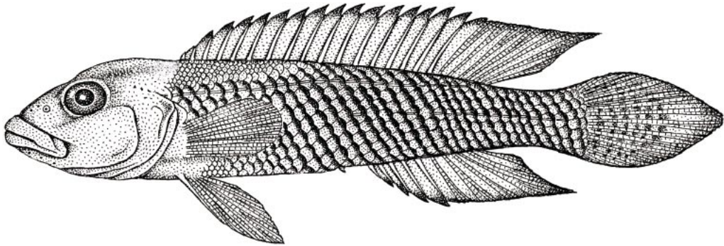
Fig. 12. Lamprologus mocquardi , AMNH 5897, male, 78 mm SL, drawn by Patricia Wynne.
