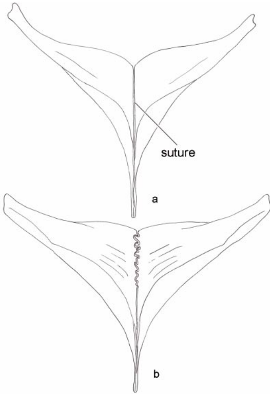
Fig. 1. Schematic of lower pharyngeal jaw ventral suture: (a) no interdigitation; (b) strongly interdigitating.
