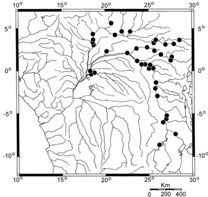
Fig. 14. Collection localities of Lamprologus mocquardi .
