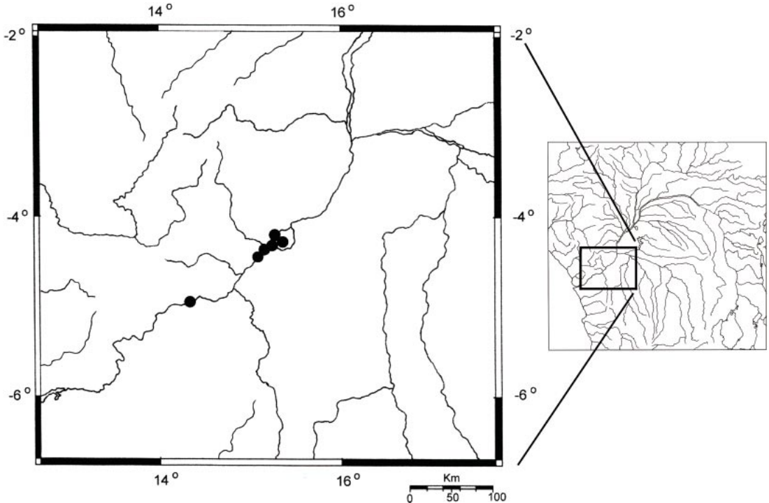
Fig. 17. Collection localities of Lamprologus wernerii .
