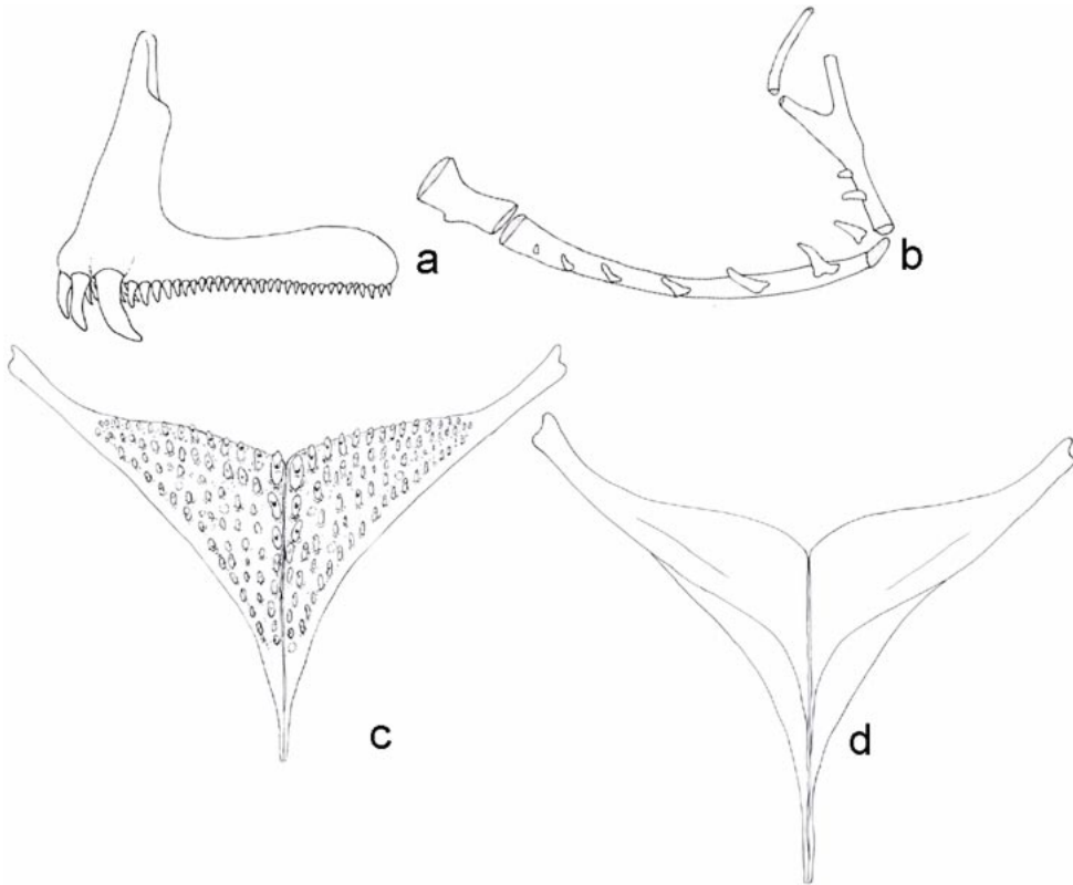
Fig. 25. Lamprologus teugelsi , n.sp., AMNH 233612: (a) premaxilla; (b) first gill arch; (c) lower pharyngeal jaw dorsal view; (d) lower pharyngeal jaw ventral view.
