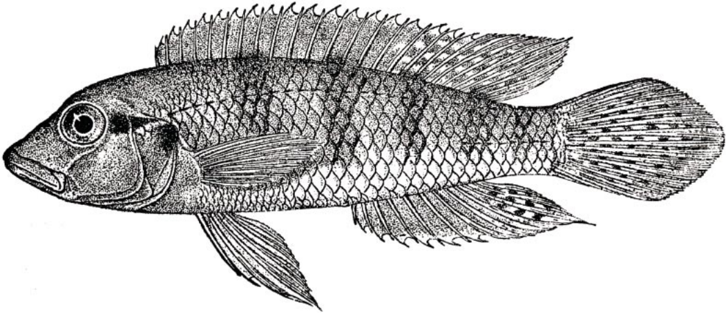
Fig. 5. Lamprologus congoensis , male, 100 mm TL, modified from Boulenger (1915).
