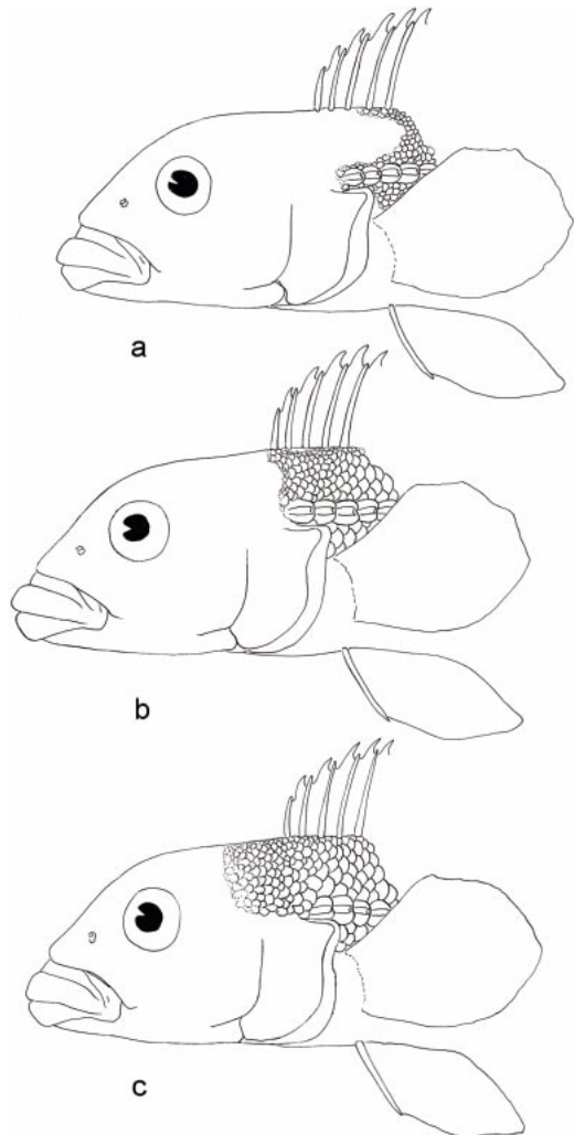
Fig. 4. Schematic of nape squamation patterns: (a) scaleless patch extends posteriorly well beyond dorsal fin origin; (b) nape scales extend anteriorly to dorsal fin origin; (c) nape scales extend anteriorly well beyond dorsal fin origin.
