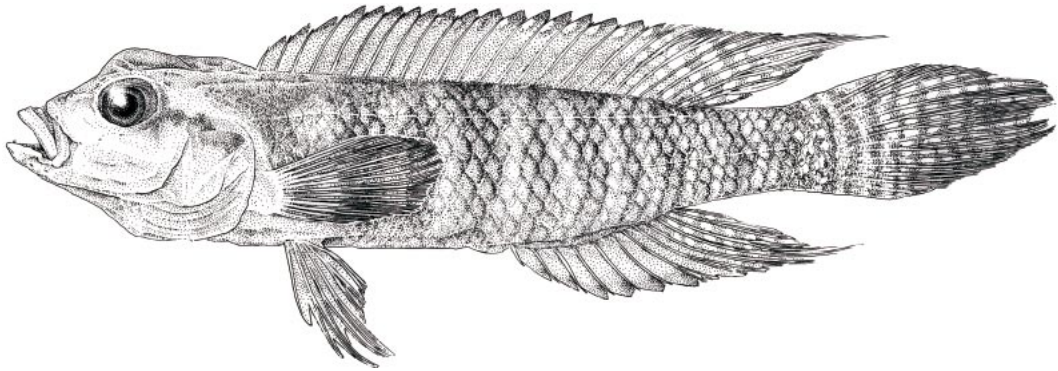
Fig. 28. Lamprologus tigripictilis , n.sp., holotype, AMNH 233609, male, 62 mm SL, drawn by Ian Hart.
