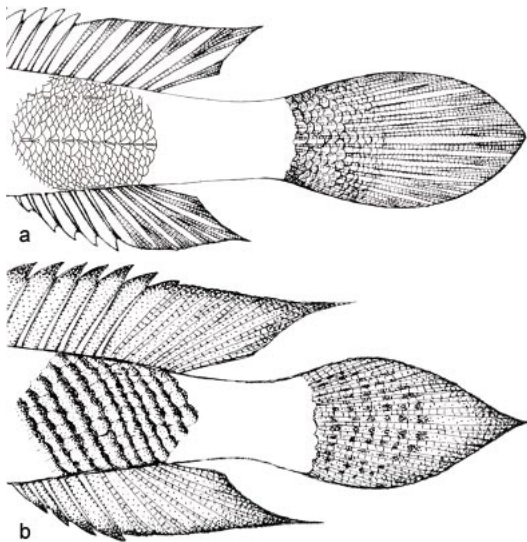
Fig. 3. Schematic of flank squamation patterns: (a) scales of irregular size, such that parallel oblique rows are obscured; (b) scales of uniform size, forming parallel oblique rows.
