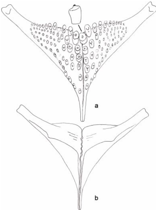
Fig. 6. Lower pharyngeal jaw of Lamprologus congoensis MRAC 78144: (a) dorsal view, showing medial molariform teeth; (b) ventral view, showing interdigitating suture.
