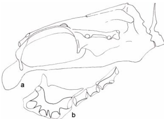
Fig. 13. Lamprologus mocquardi , AMNH 5828: (a) neurocranium and first vertebra; (b) lachrymal and adjacent infraorbitals.
